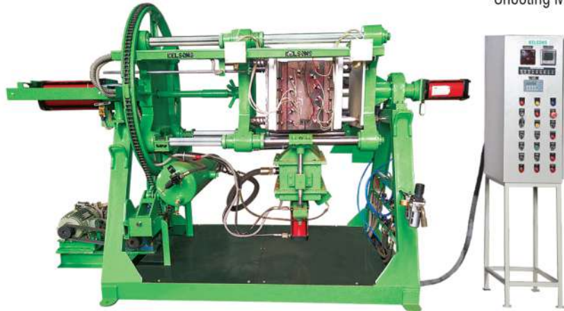
Rollover Vertical Parting Shooting Machine
